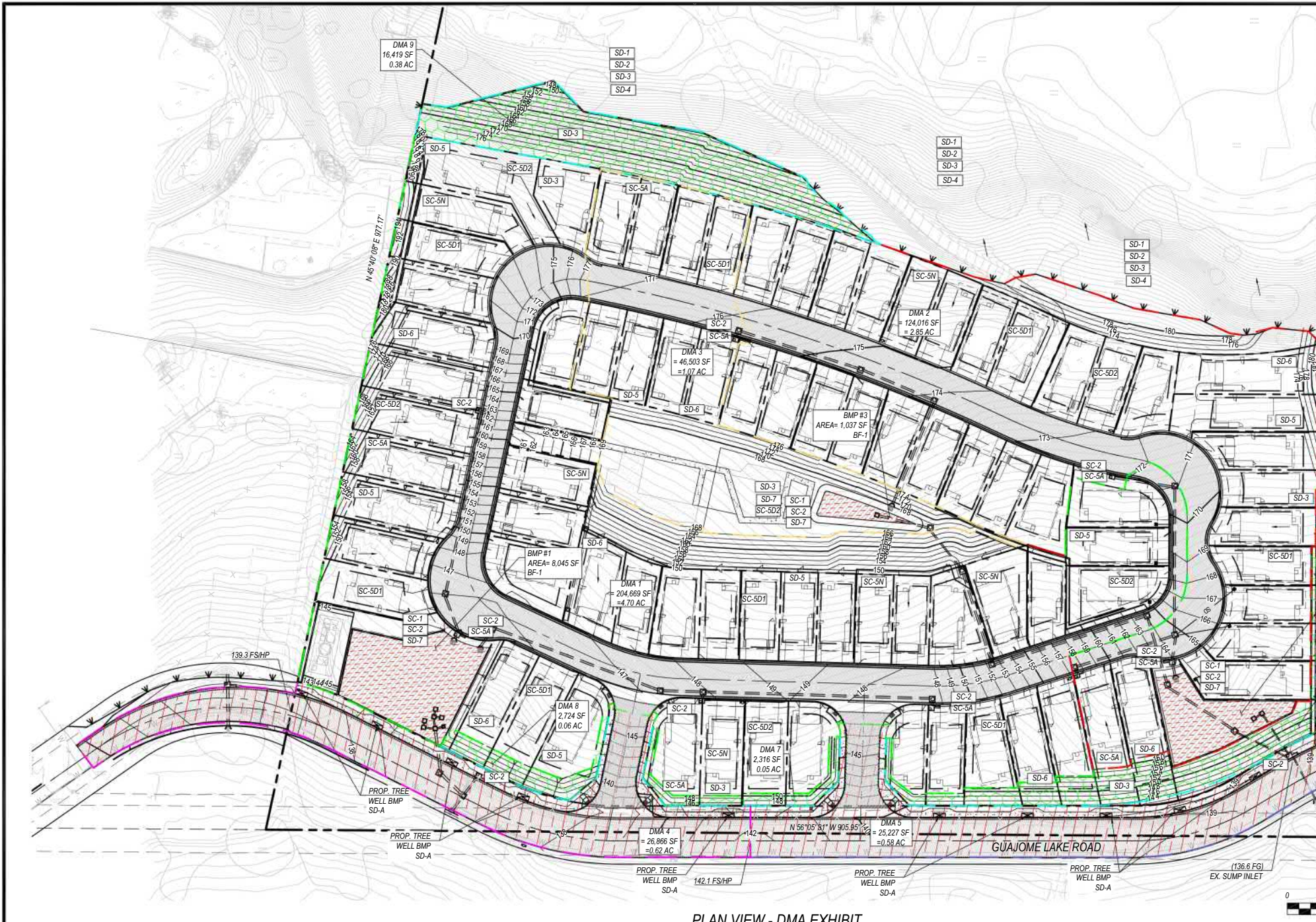
PLAN VIEW - DMA EXHIBIT SCALE: 1" = 50'
