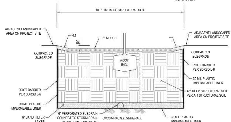
SECTION A-A TREE WELL W/O GRATE MODIFIED SDC GS DS SD-1.04A + GS-1.04B
