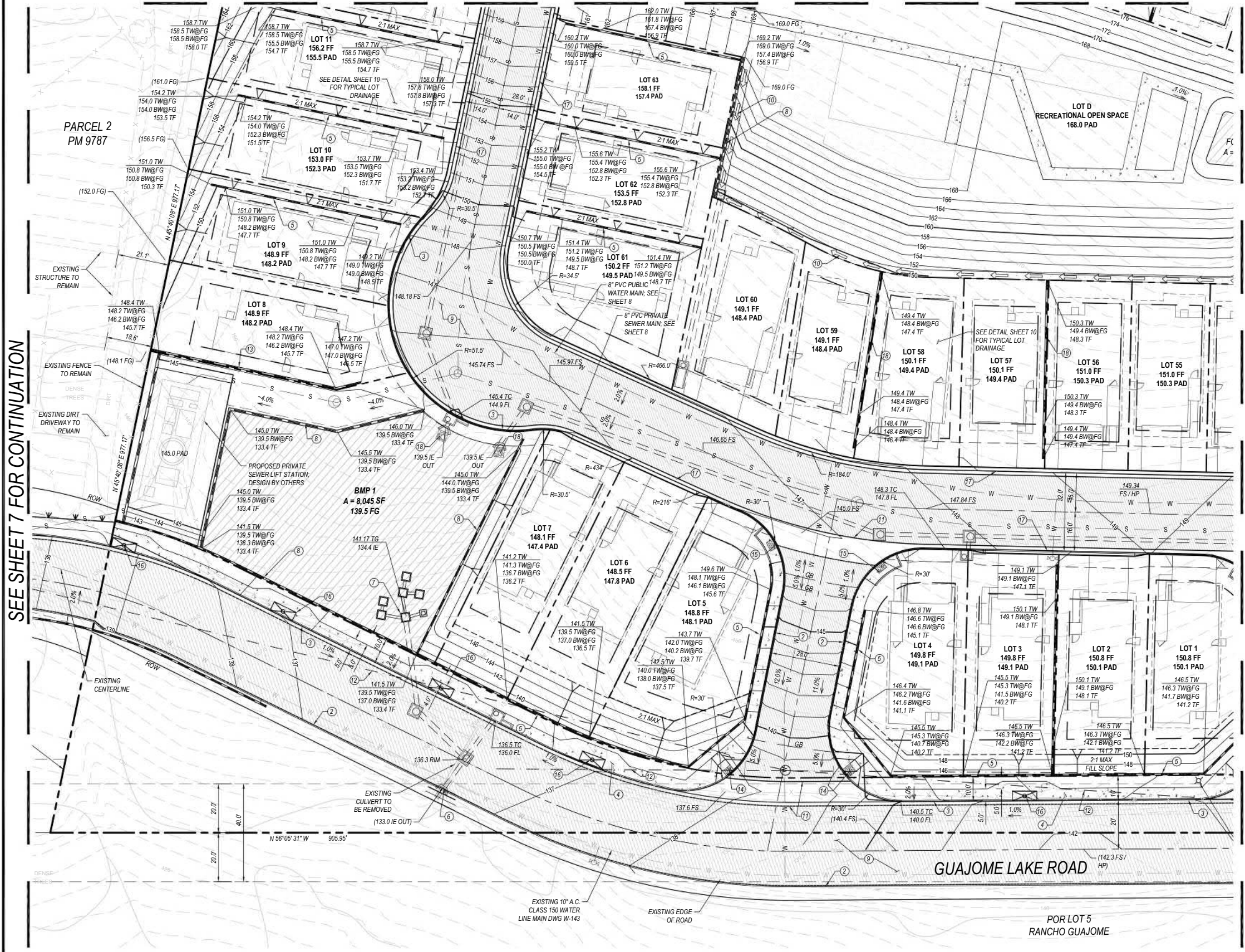
PLAN VIEW - PRELIMINARY GRADING PLAN SCALE: 1" = 20'
