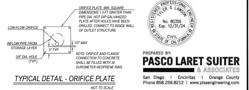
TYPICAL DETAIL - ORIFICE PLATE NOT TO SCALE
