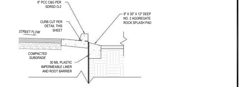
SECTION C-C CURB CUT @ TREE WELL SDC GS DS GS 5.01 NOT TO SCALE
