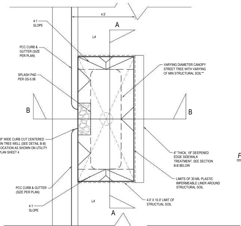
PLAN VIEW - CURB CUT @ TREE WELL SDC GS DS GS-5.01
