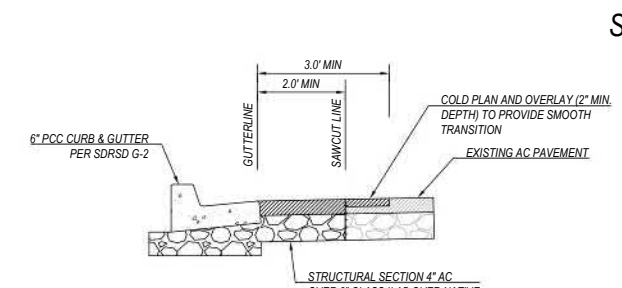
TYPICAL DETAIL - AC PAVEMENT SAWCUT SCALE: NTS
