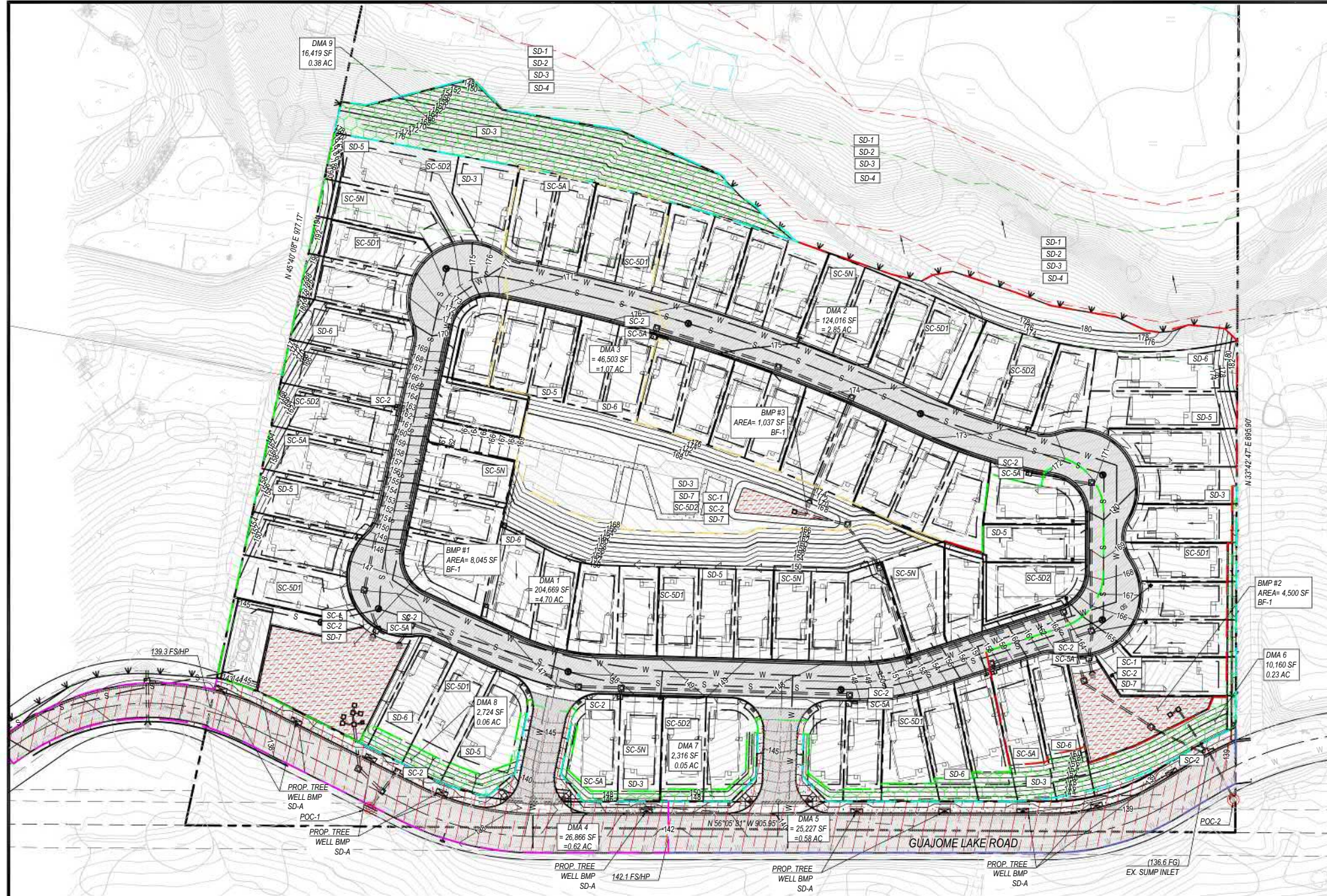
PLAN VIEW - HMP EXHIBIT SCALE: 1" = 50'
