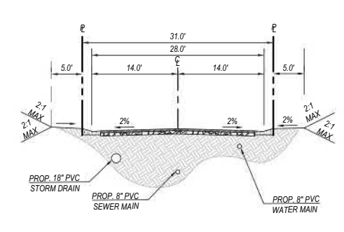
TYPICAL SECTION - PRIVATE ROAD NORTH SCALE: NTS
