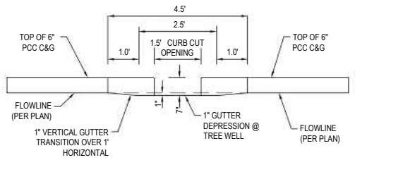
SECTION D-D CURB CUT @ TREE WELL SDC GS DS GS 5.01
