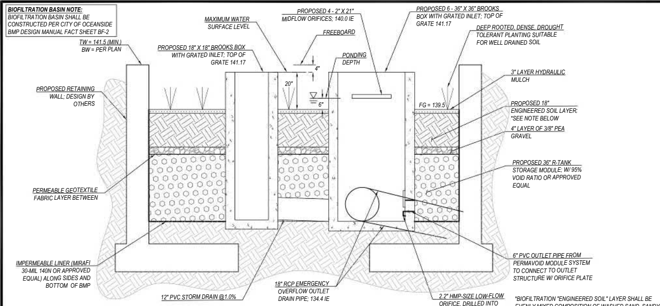
TYPICAL DETAIL - BMP 1 BIOFILTRATION BASIN
