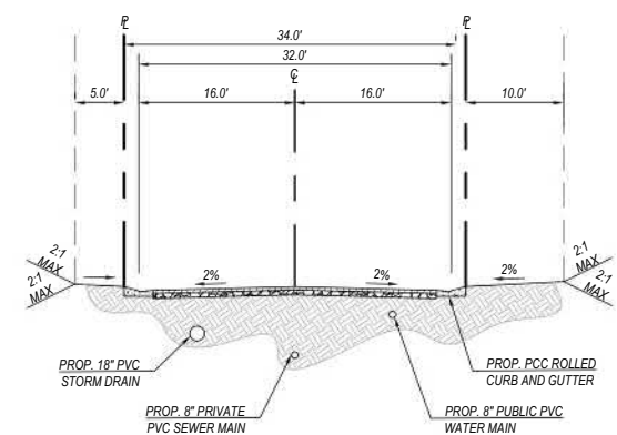
TYPICAL SECTION - PRIVATE ROAD SOUTH SCALE: NTS
