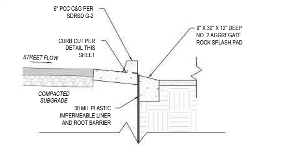
SECTION C-C CURB CUT @ TREE WELL SDC GS DS GS 5.01
