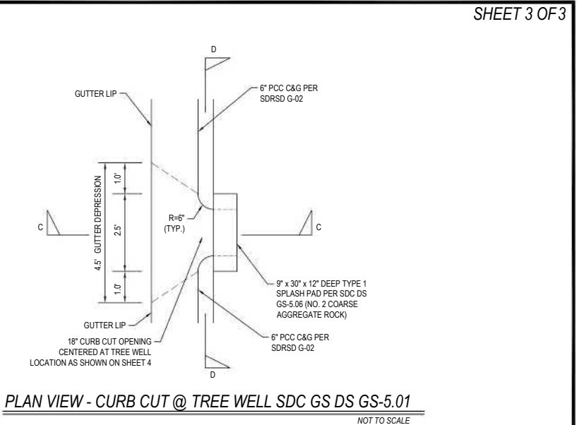
PLAN VIEW - CURB CUT @ TREE WELL SDC GS DS GS-5.01 NOT TO SCALE
