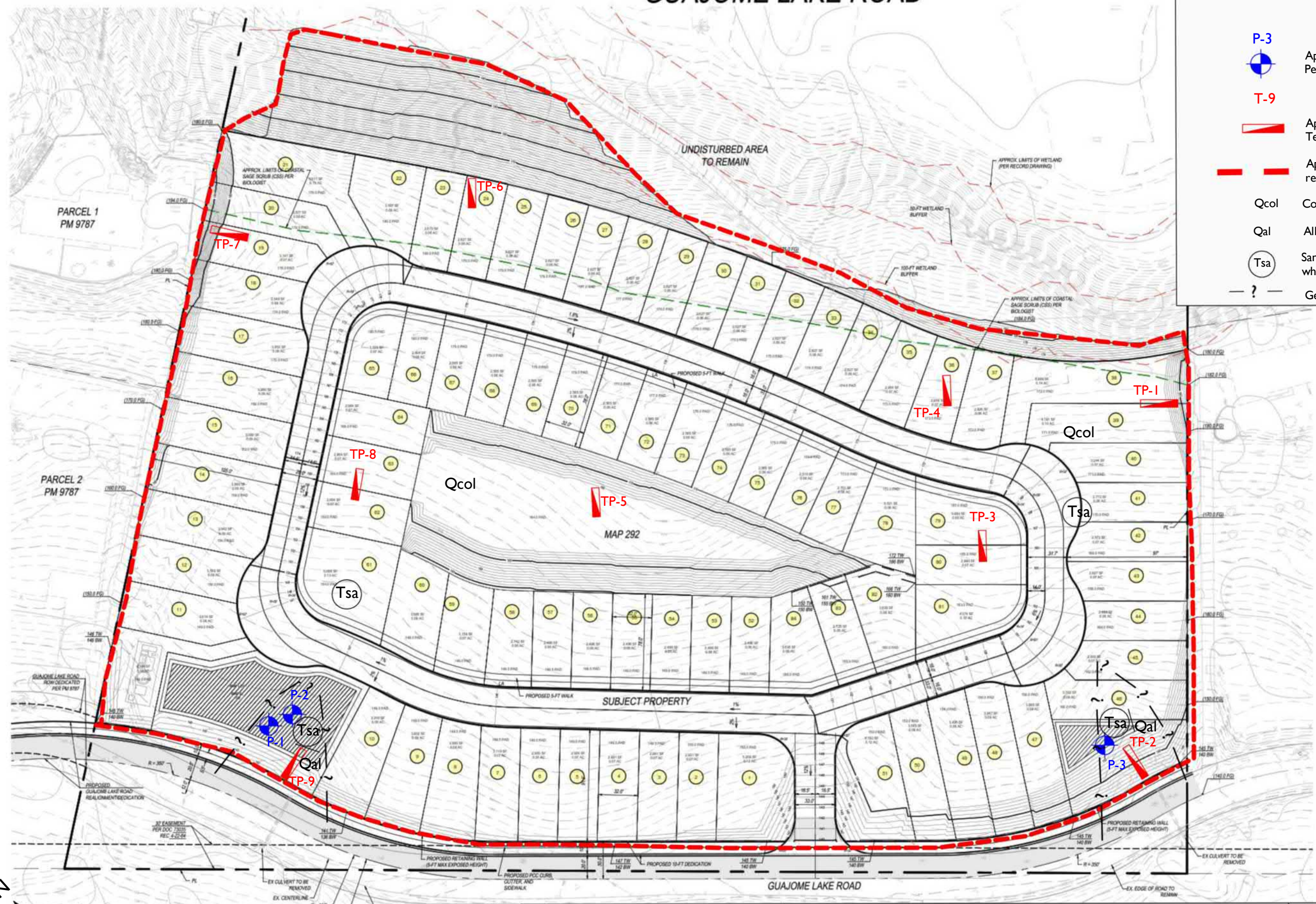
Figure 2 Geotechnical Map
