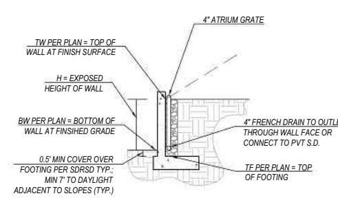
TYPICAL DETAIL - RETAINING WALL SCALE: NTS
