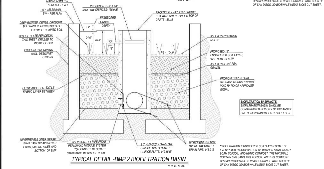
TYPICAL DETAIL - BMP 2 BIOFILTRATION BASIN NOT TO SCALE
