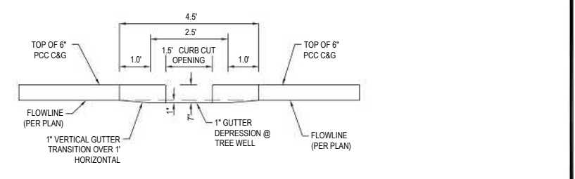
SECTION D-D CURB CUT @ TREE WELL SDC GS DS GS 5.01 NOT TO SCALE
