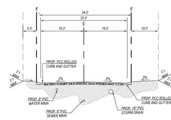
TYPICAL SECTION - PRIVATE ROAD WEST SCALE: NTS
