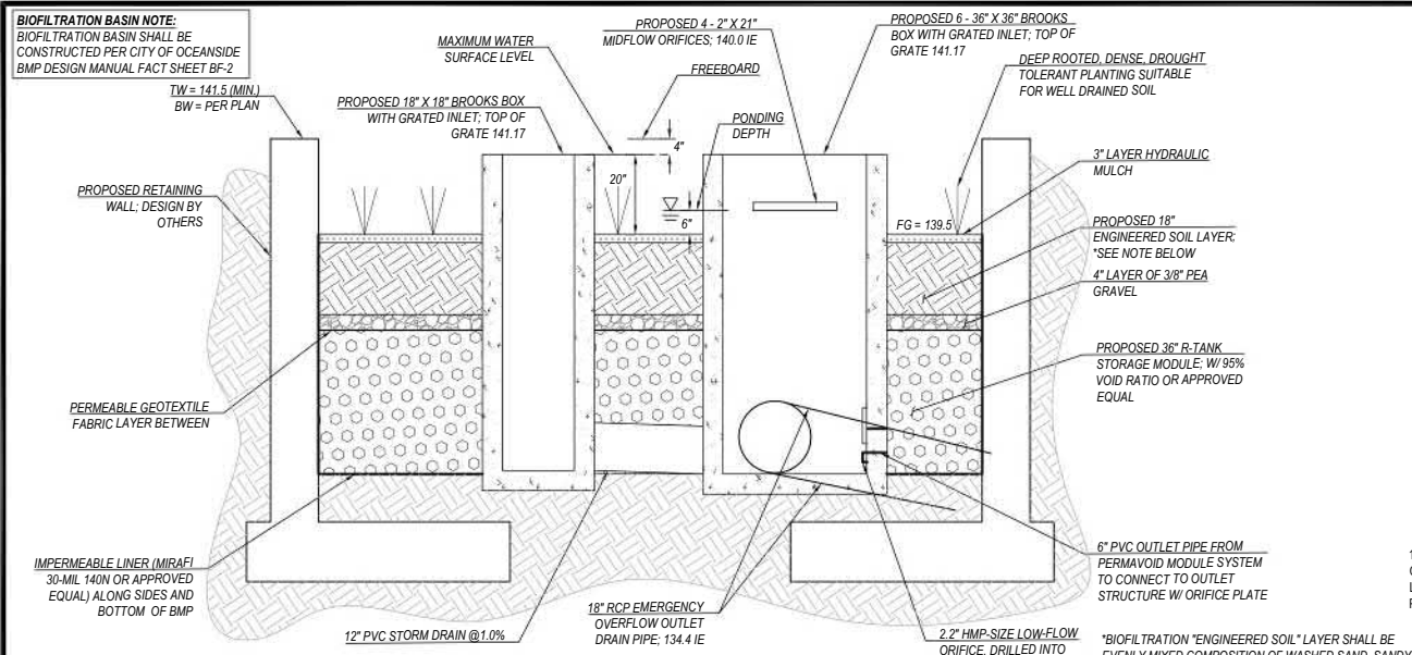
TYPICAL DETAIL - BMP 1 BIOFILTRATION BASIN SCALE: NTS
