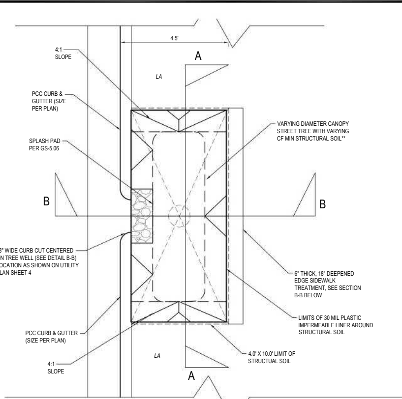
PLAN VIEW - CURB CUT @ TREE WELL SDC GS DS GS-5.01 NOT TO SCALE
