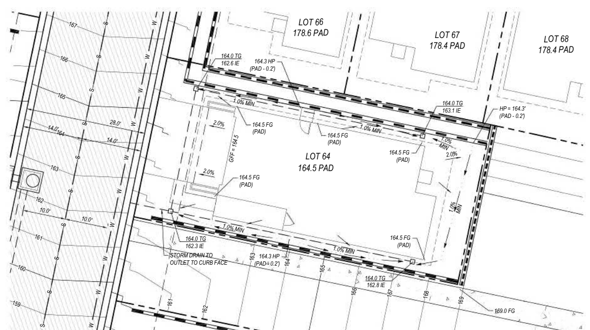
TYPICAL DETAIL - LOT DRAINAGE FOR PRELIMINARY PRECISE GRADING SCALE: 1" = 10'
