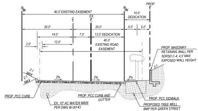
TYPICAL SECTION - GUAJOME LAKE ROAD SCALE: NTS
