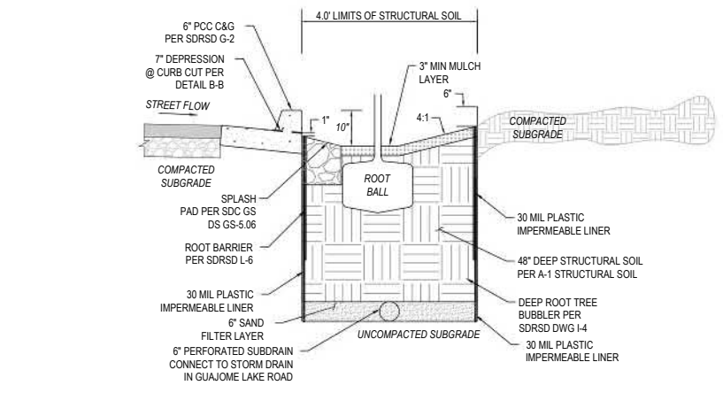
SECTION B-B TREE WELL W/O GRATE MODIFIED SDC GS DS SD-1.04A + GS-1.04B NOT TO SCALE
