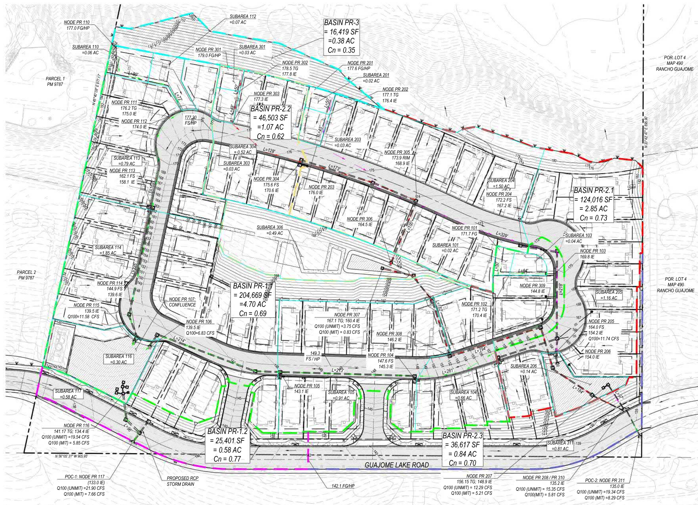
PLAN VIEW - PROPOSED HYDROLOGY NODE MAP SCALE: 1" = 40' HORIZONTAL
