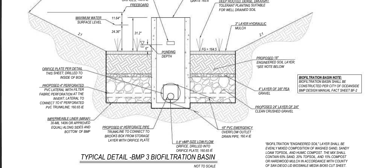
TYPICAL DETAIL - BMP 3 BIOFILTRATION BASIN NOT TO SCALE
