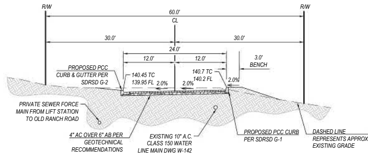
SECTION CUT X-X NOT TO SCALE
