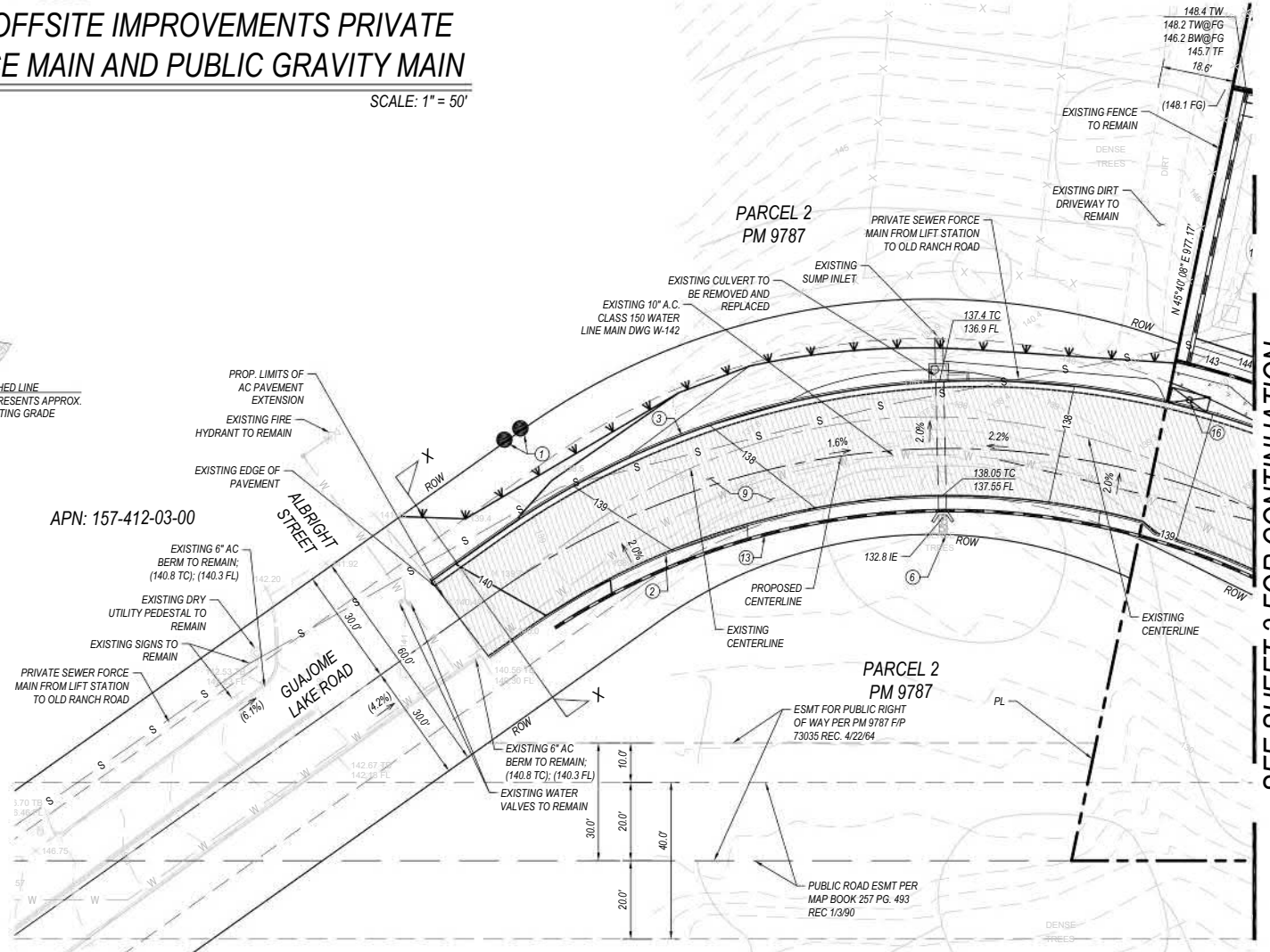
PLAN VIEW - PRELIMINARY GRADING PLAN
