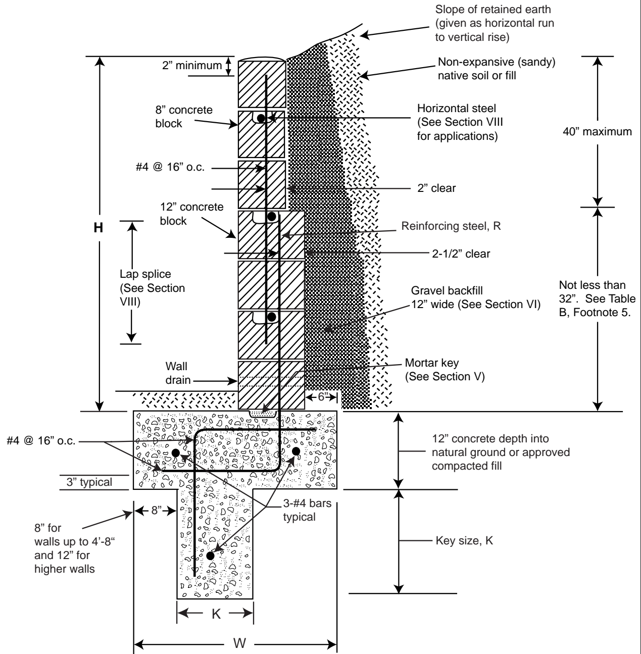
Figure 2 Type II retaining wall with sloping backfill
